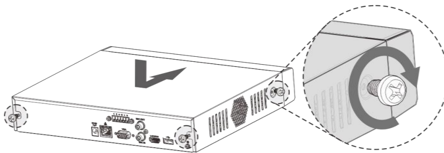
Figure 2-6 Installing HDD (6)
