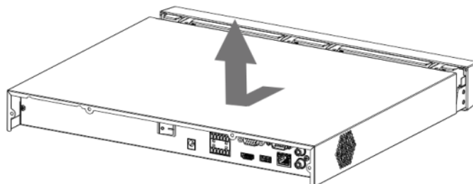
Figure 2-8 Installing HDD (2)
