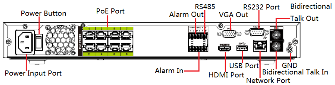
Figure 3-1 Connection sample
