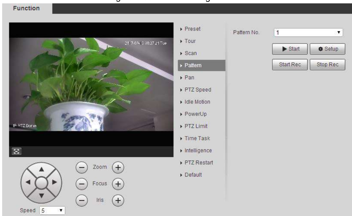
Figure 5-69 Pattern settings
