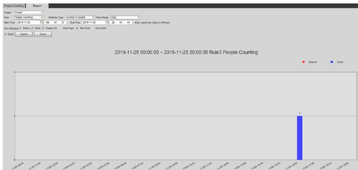
Figure 5-110 People counting—report
