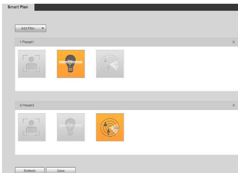
Figure 5-88 Smart plan (3)
