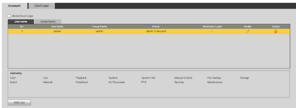
Figure 5-139 Account interface
