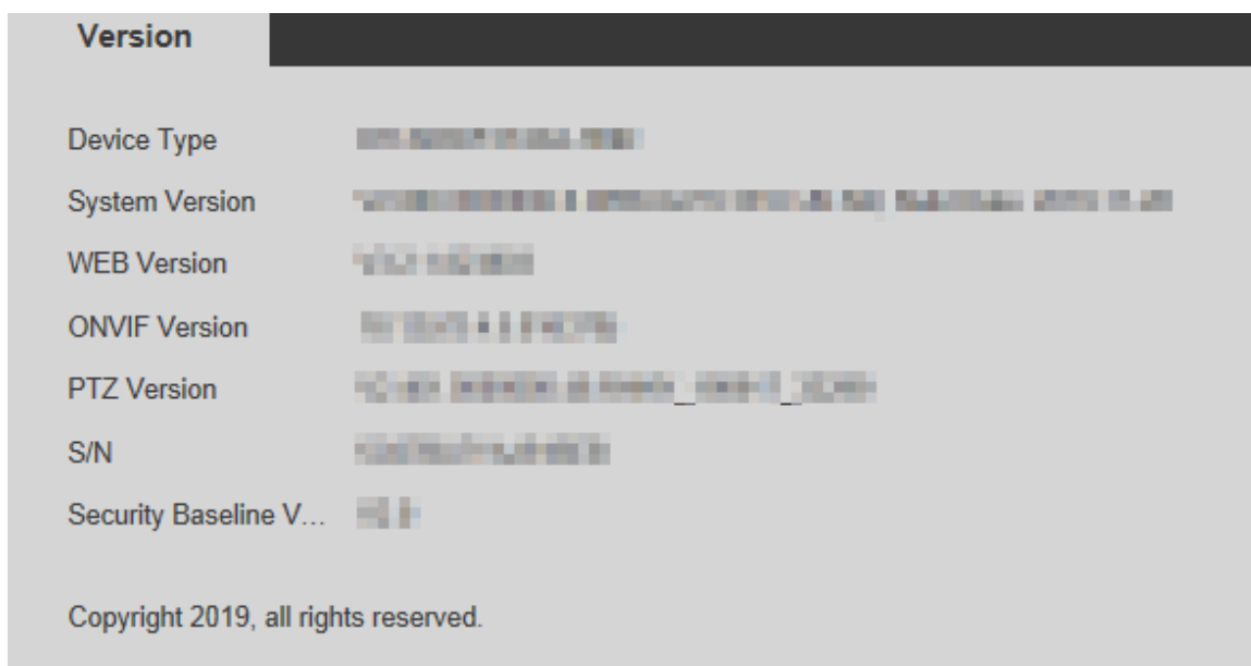
Figure 5-166 Version
