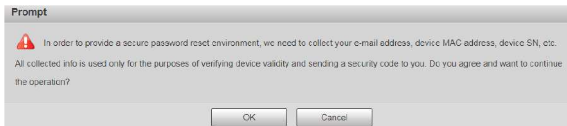
Figure 1-13 Prompt
