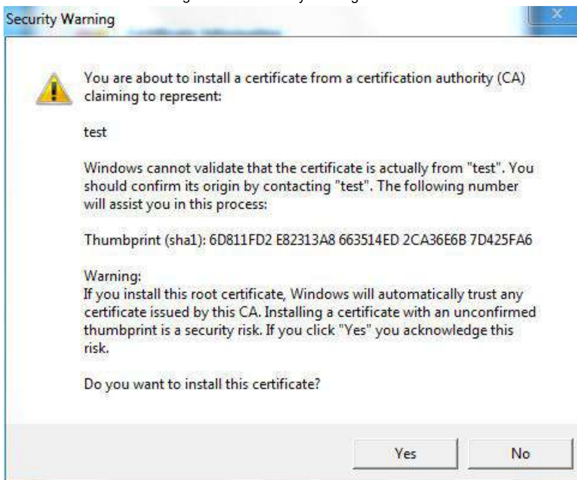
Figure 5-156 Security warning
