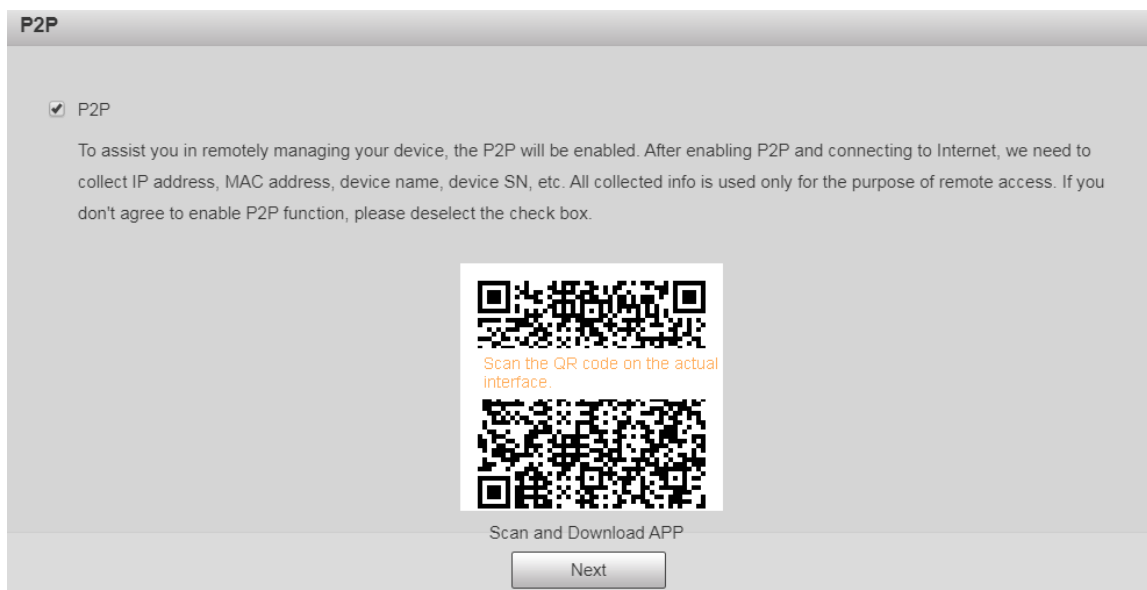
Figure 1-6 P2P interface
