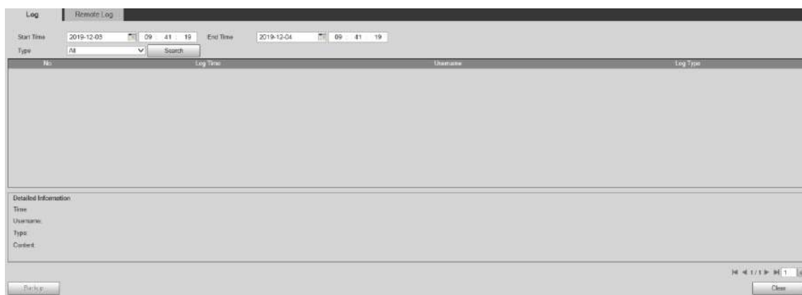
Figure 5-167 Log
