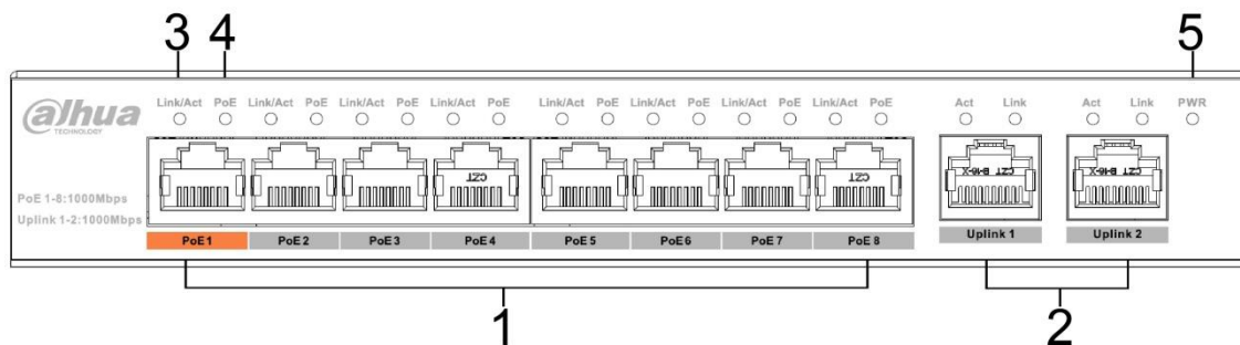
Figure 2-1 Front panel
