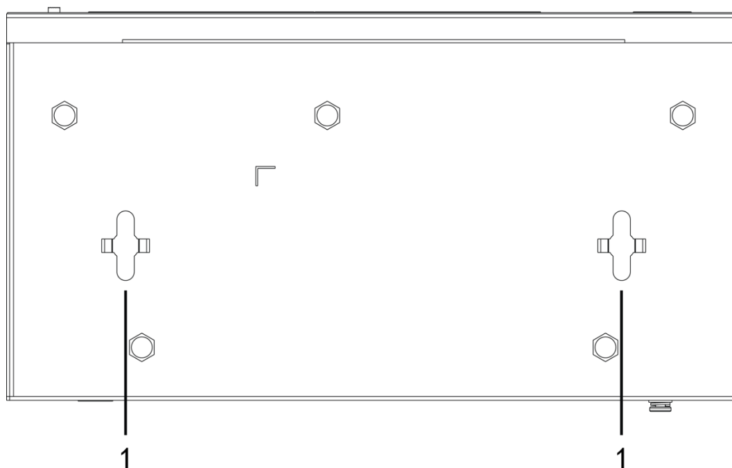
Figure 2-3 Side panel
