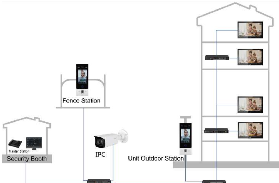
Figure 2-1 Cable connection
