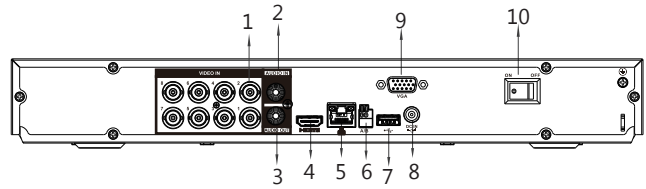
DH-XVR5208AN-4KL-X-8P
