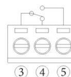
COM NC NO ALARM
