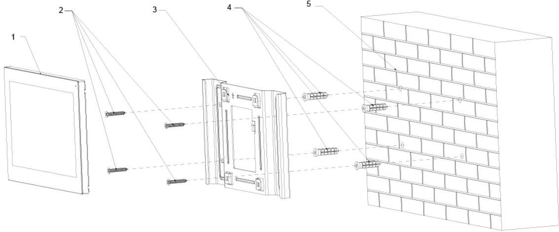
Figure 2-1 Installation
