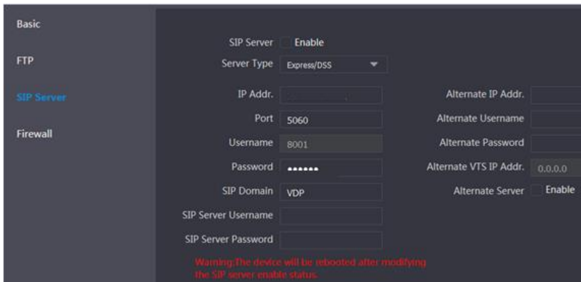
Figure 4-8 SIP server (2)
