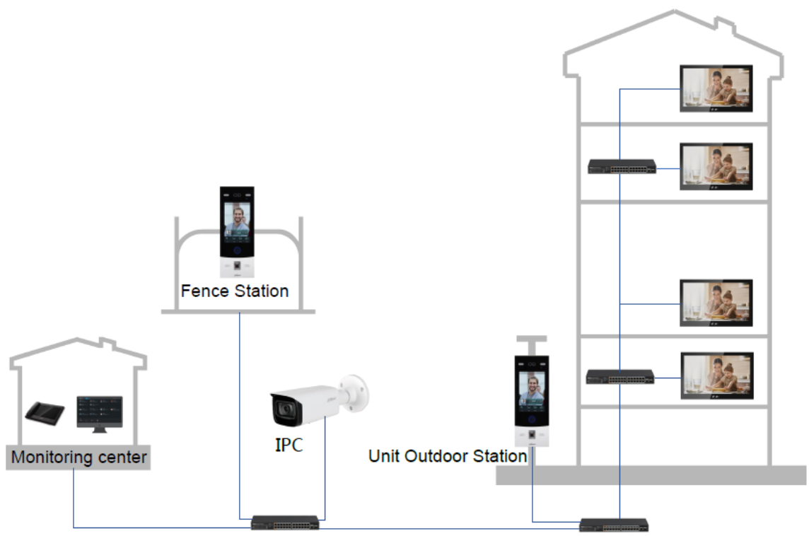
Figure 3-1 Network diagram
