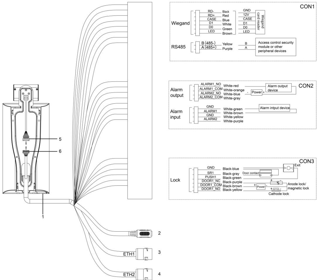
Figure 2-1 Cable connections
