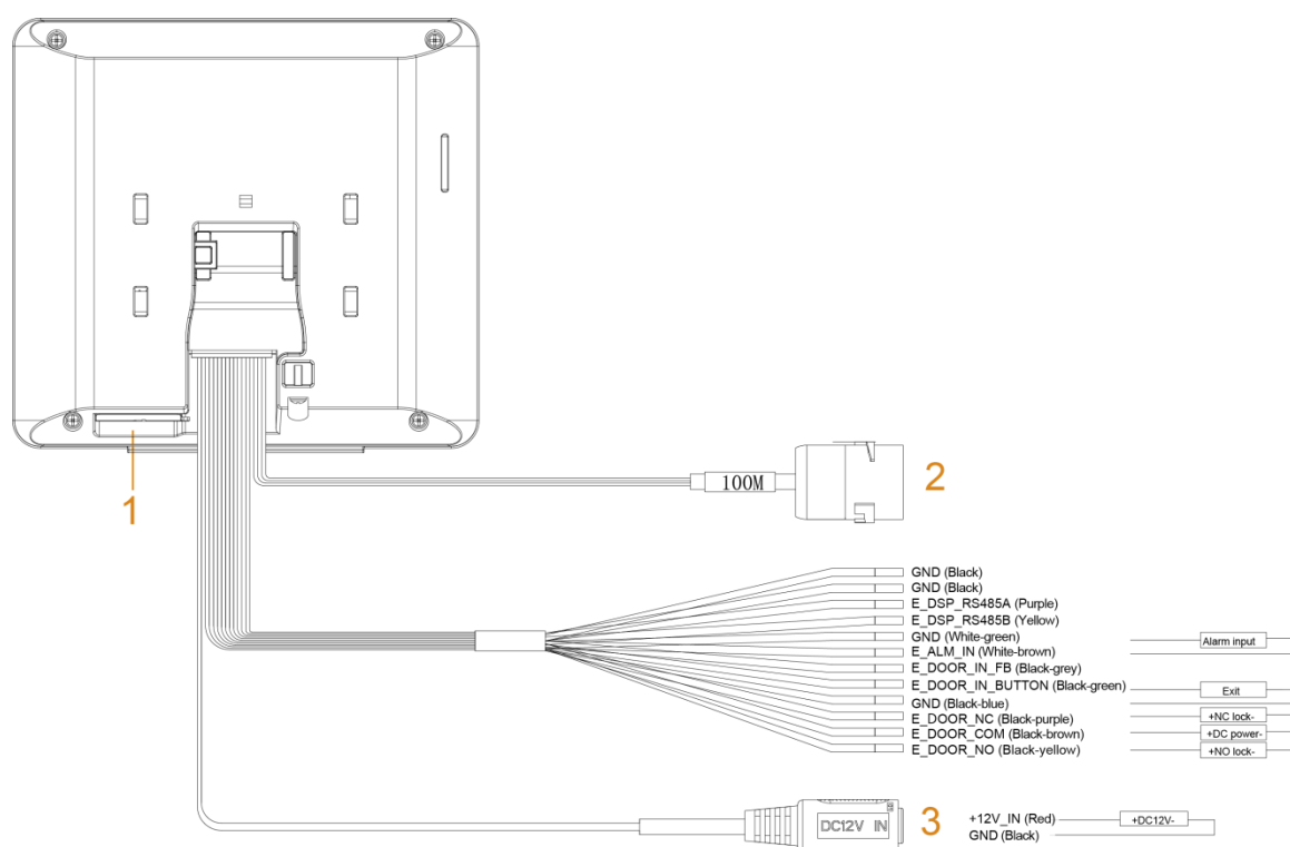
Figure 2-1 Cable connection
