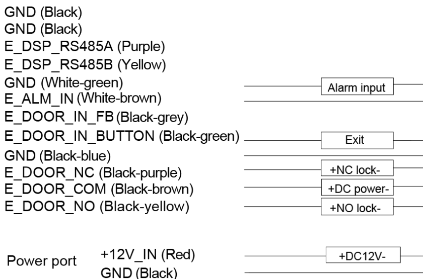
Figure 2-2 Ports
