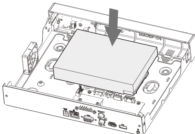
Figure 2-9 Installing HDD (3)
