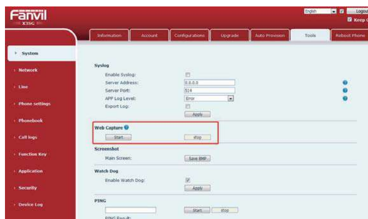
Picture 138 - Screenshot
