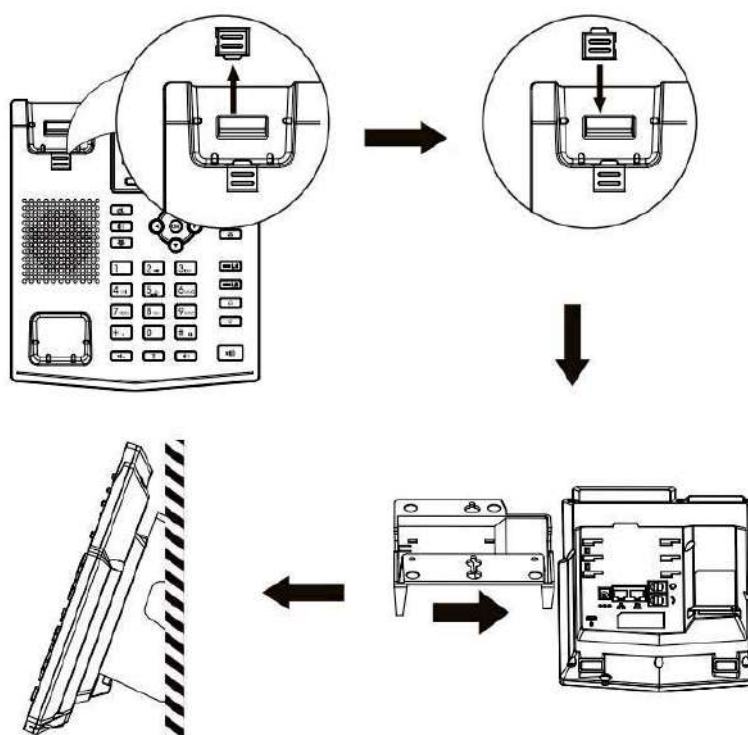
Picture 2 - Wall-mounted installation
