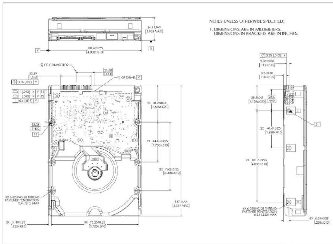
Figure 2-1. Mounting Dimensions
