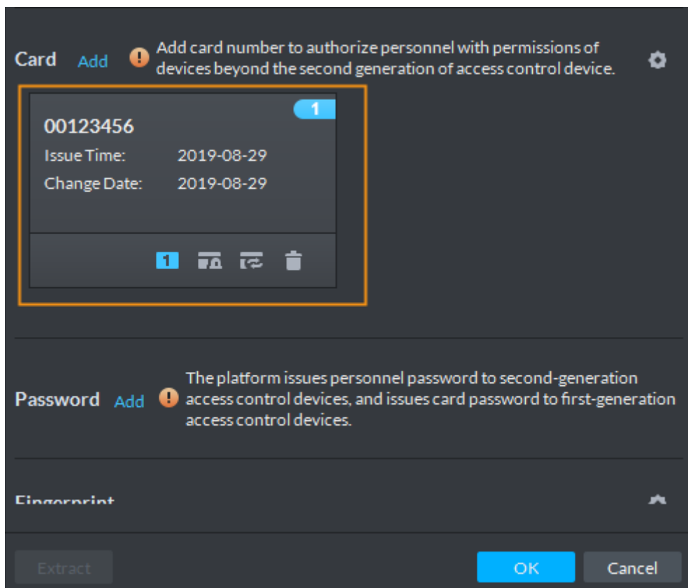
Figure 4-6 Added card
