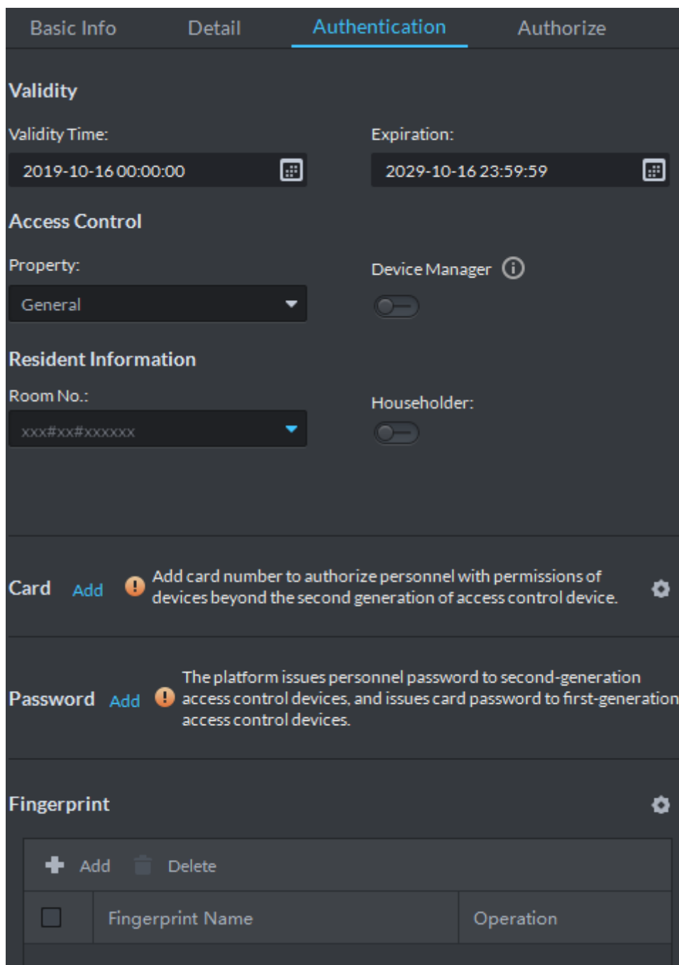
Figure 4-4 Authentication
