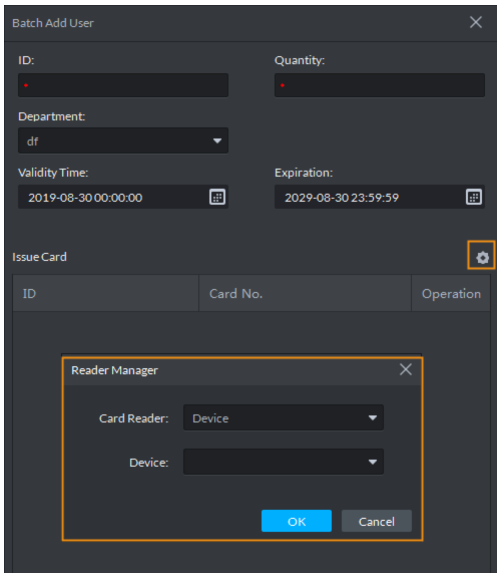
Figure 4-18 Reader manager
