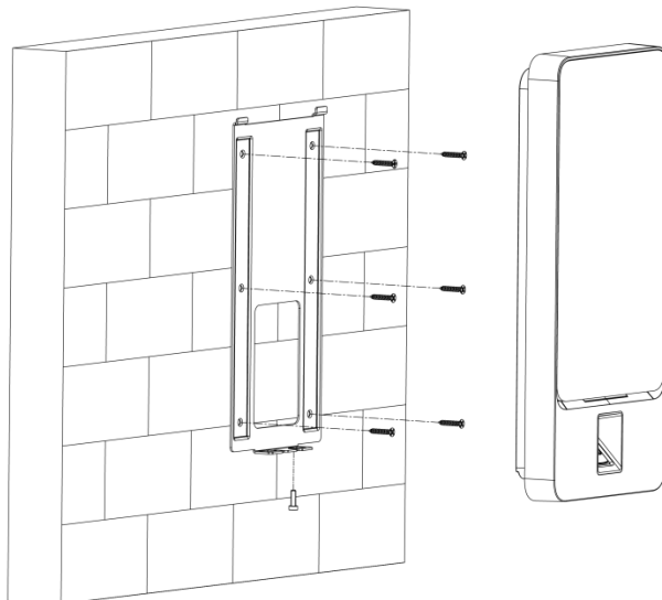
Figure 2-2 Installation diagram (1)
