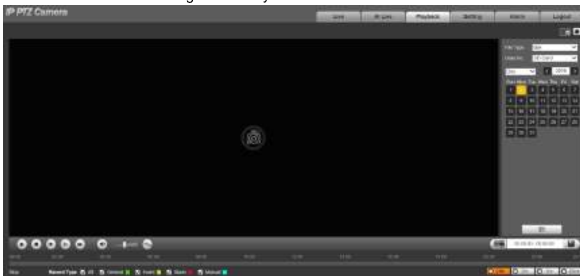
Figure 4-1 Playback interface
