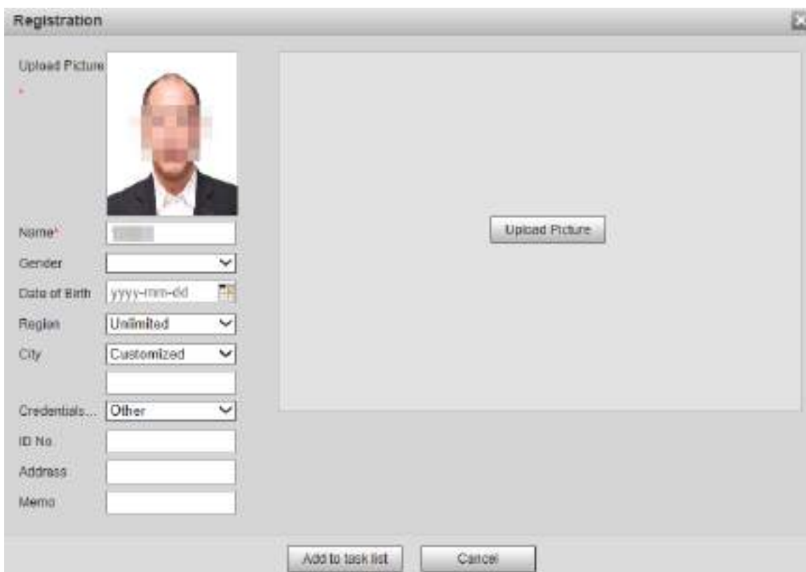
Figure 5-103 Registration interface
