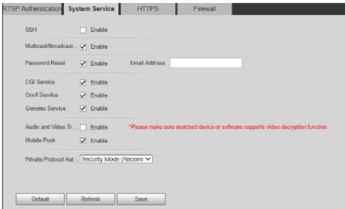
Figure 5-145 System service
