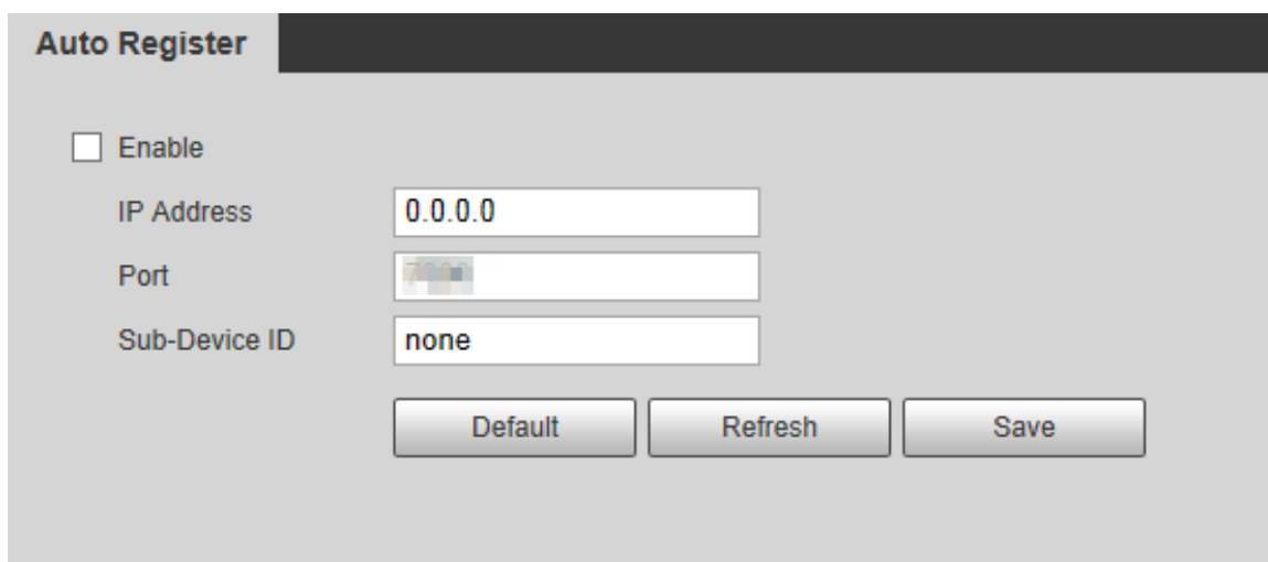
Figure 5-48 Auto register
