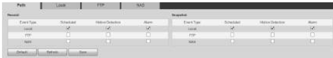
Figure 5-130 Path settings
