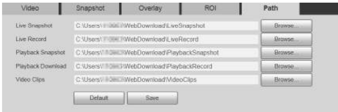
Figure 5-34 Path settings
