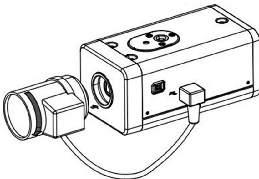
Figure 8-1 Lens installation (1)
