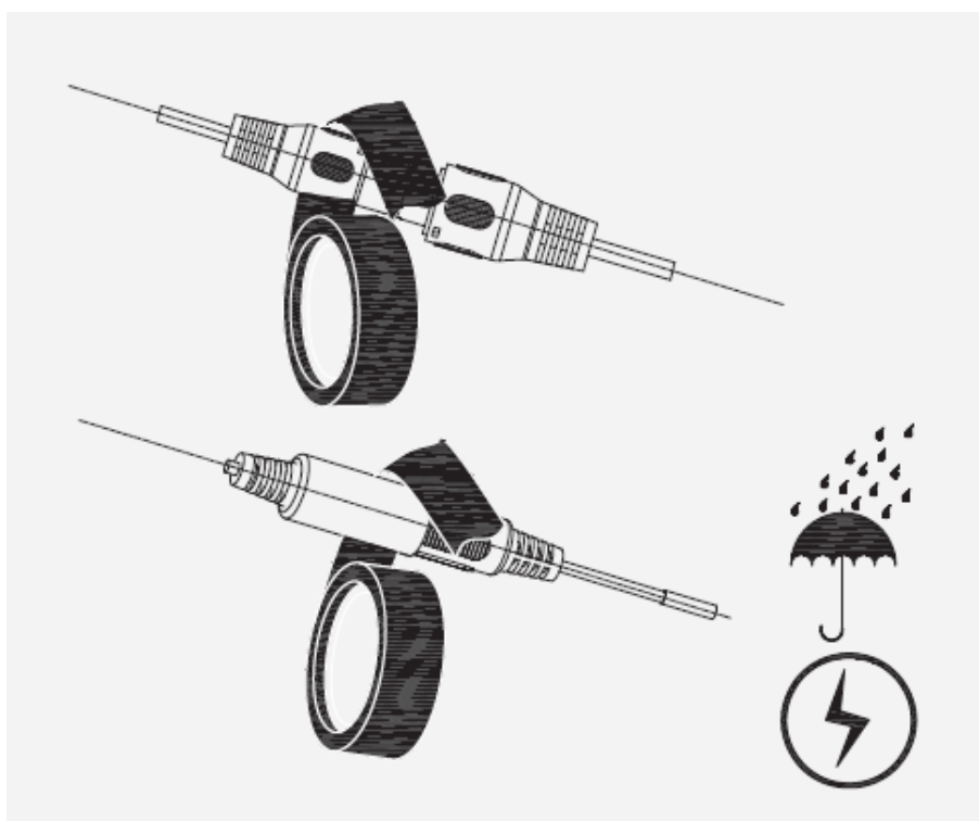
Figure 10-2 Waterproof measures
