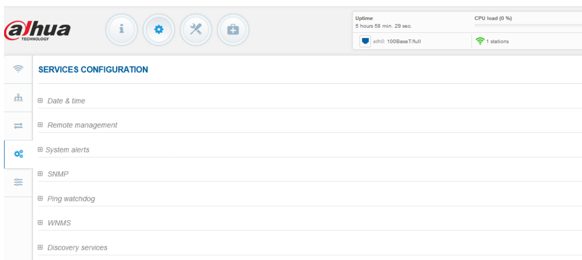
Figure 61 - Services Menu
