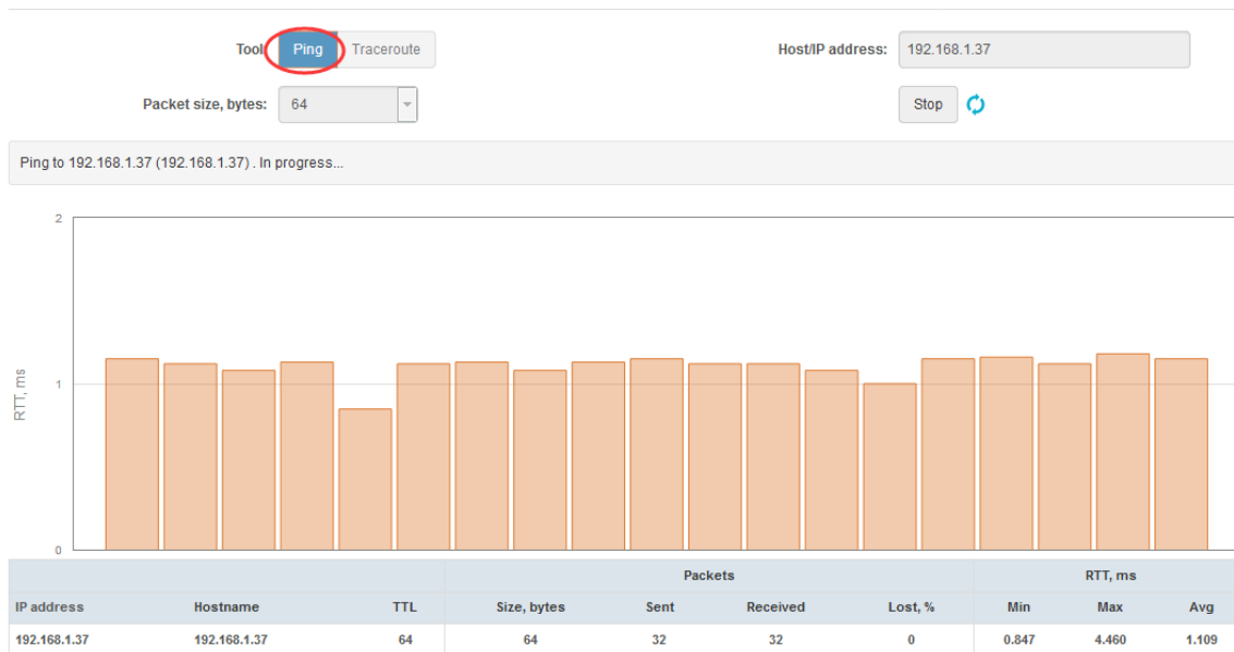
Figure 83 - Ping tool
