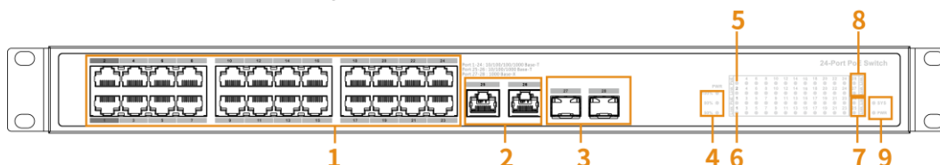
Figure 2-3 Front panel
