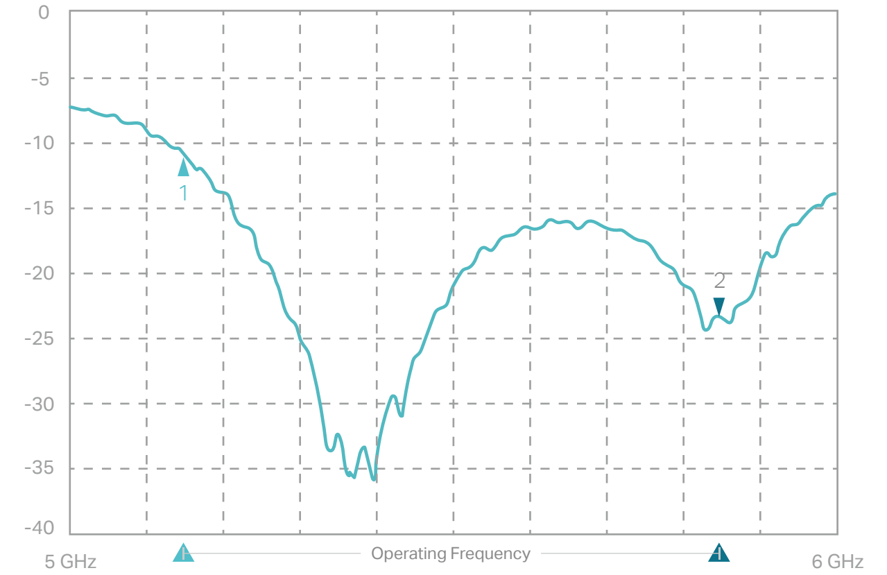
Return Loss
