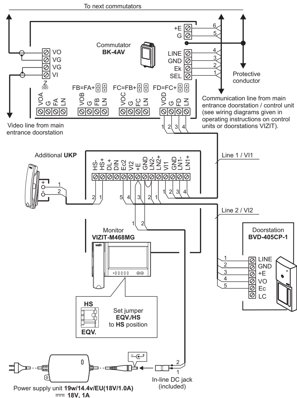
Monitor VIZIT-M468MG(MS) with commutator for multi-apartment video doorphone, 1-subscriber individual doorstation, and additional apartment handset UKP.
