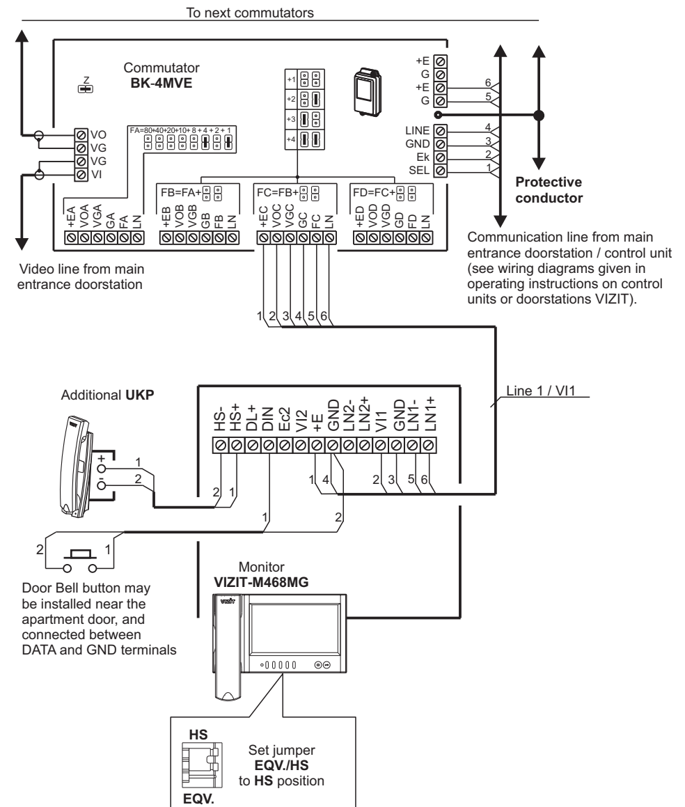
Monitor VIZIT-M468MG(MS) with commutator for multi-apartment video doorphone, additional apartment handset УКП , and Door Bell button. The Monitor is powered from a group power supply unit.
