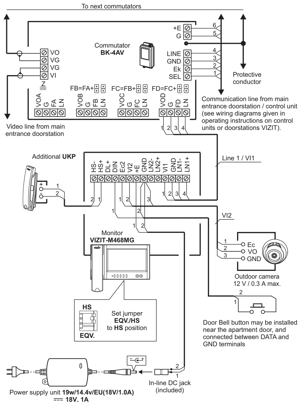
Monitor VIZIT-M468MG(MS) with commutator for multi-apartment video doorphone, additional apartment handset UKP , outdoor camera, and Door Bell button.
