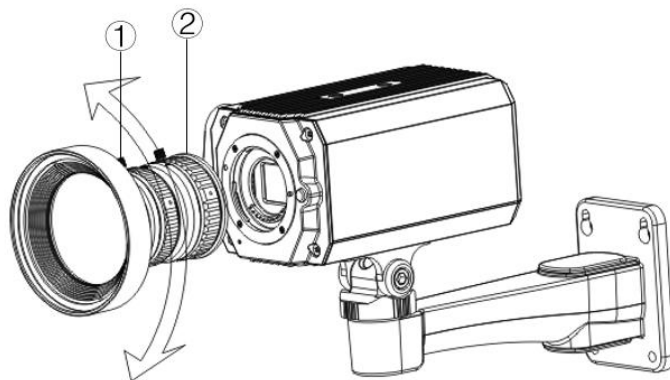
Figure 8-3 Lens installation (2)
