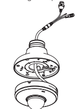
Figure 4-3 Pulling the speed dome cables
