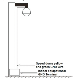
Appendix figure 1-2 Indoor installation
