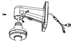
Figure 4-8 Installation position requirement
