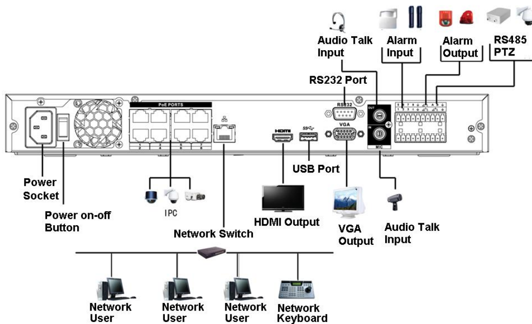
Figure 3-1 Device connection
