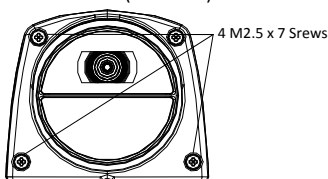
Figure 2-6 Insert Screws
