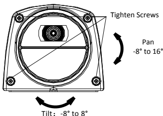
Figure 2-7 Tighten Screws and Adjust Camera
