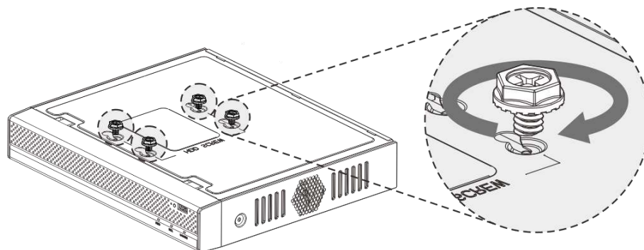
Figure 2-4 Installing HDD (4)
