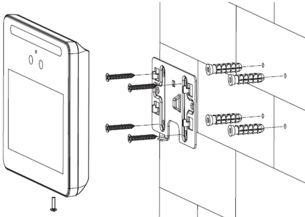
Figure 2-2 Wall installation
