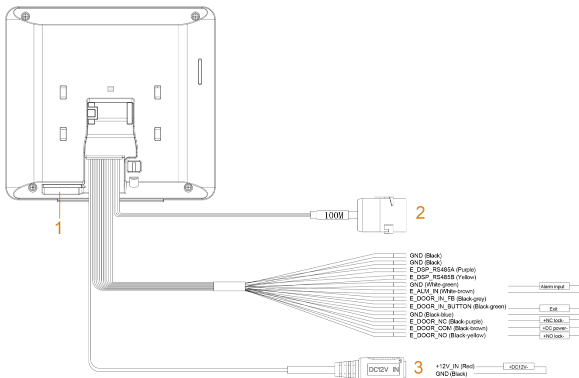
Figure 2-2 Ports
