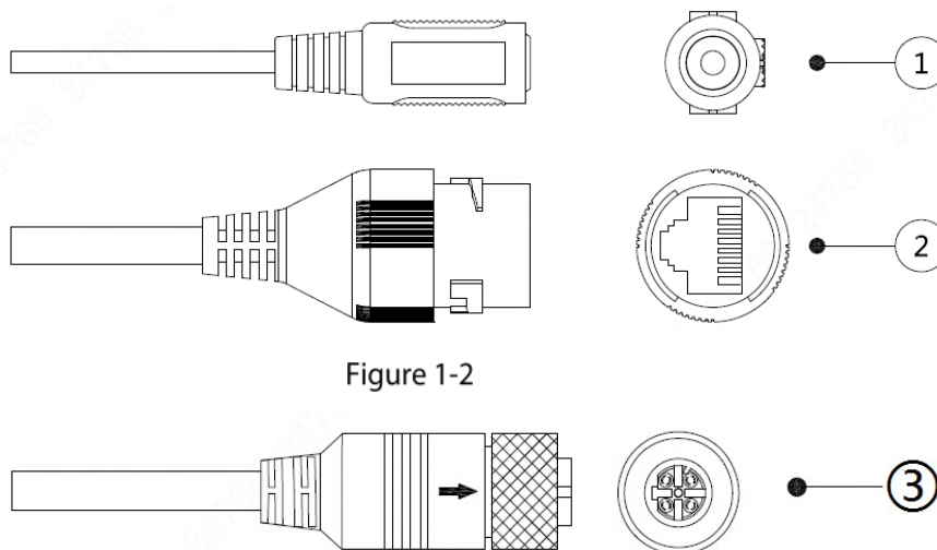
Figure 1-1 Cable list
