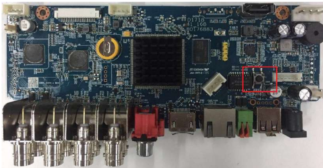
Figure 5-14 Reset button
