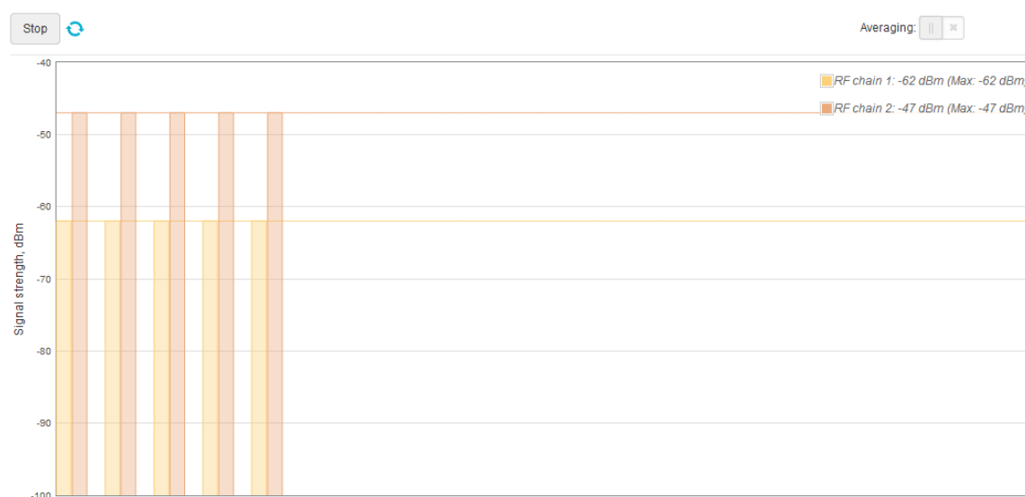
Figure 80 – Antenna Alignment
