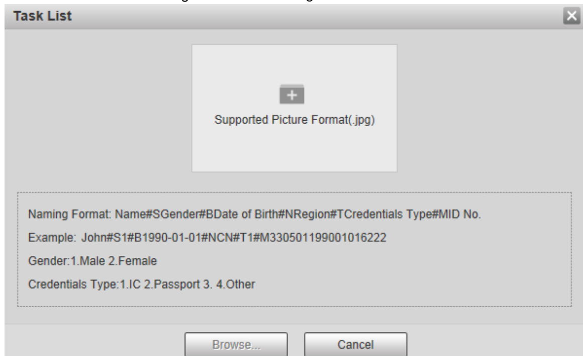
Figure 5-102 Batch registration
