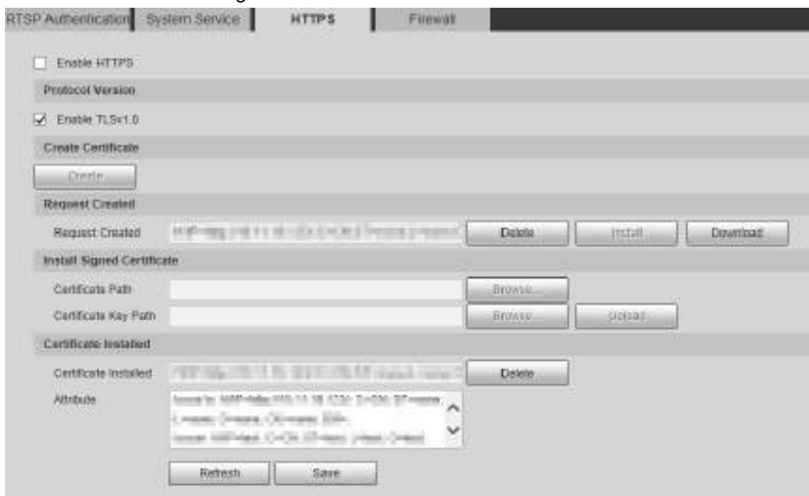
Figure 5-150 Certificate installation
