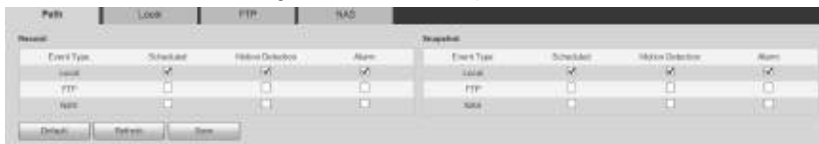
Figure 5-132 Path settings
