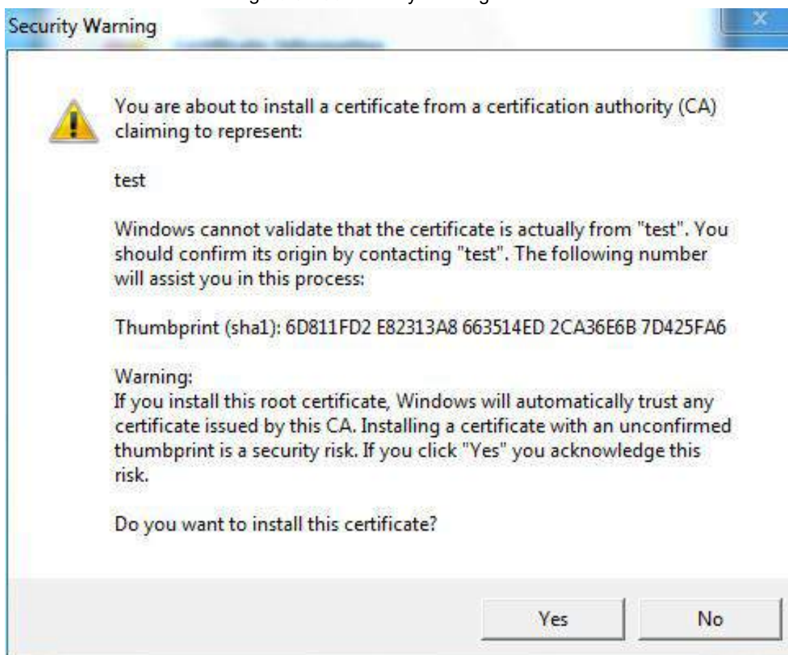
Figure 5-156 Security warning
