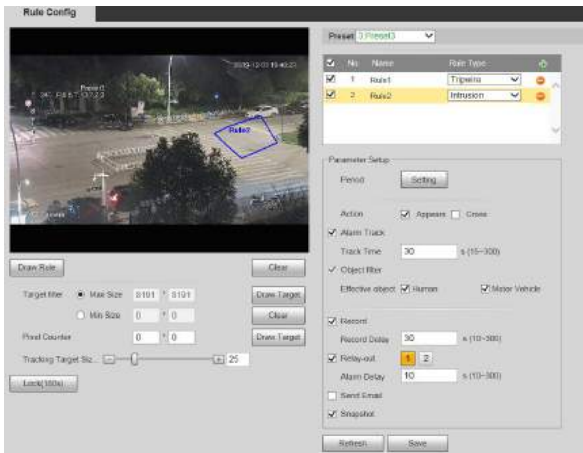
Figure 5-91 Intrusion settings
