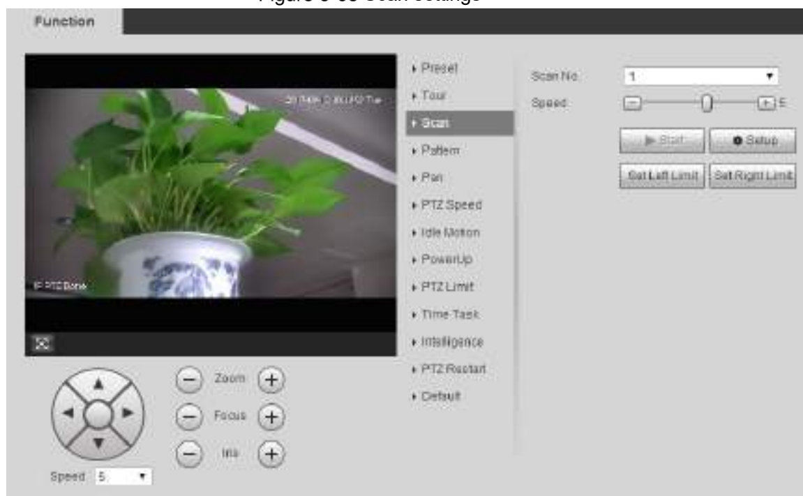
Figure 5-68 Scan settings
