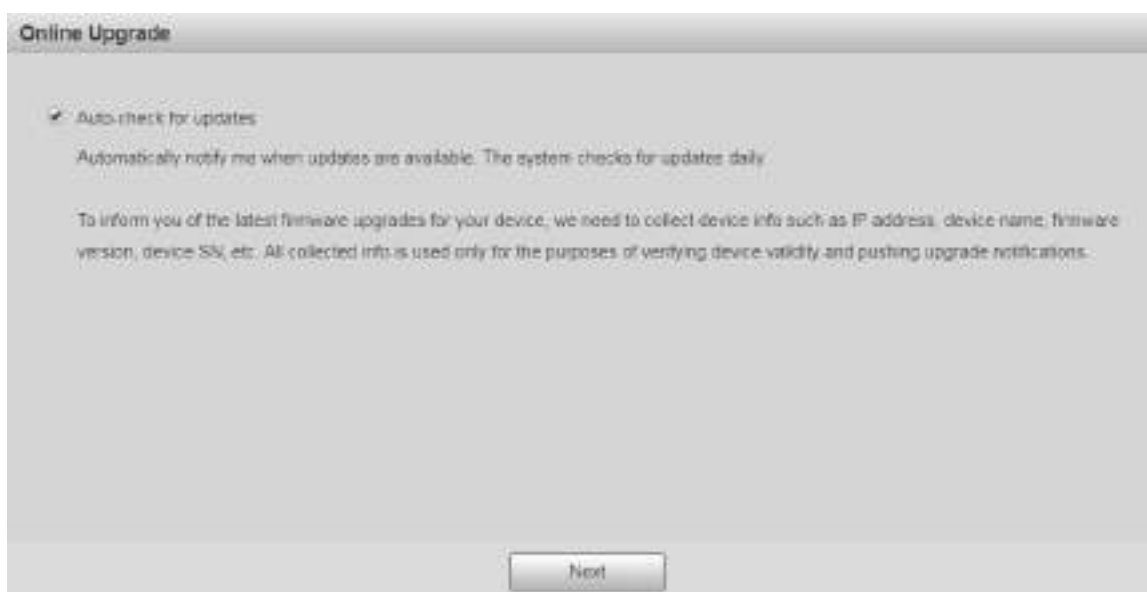
Figure 1-7 Online upgrade
