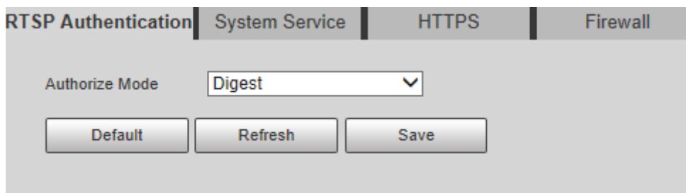
Figure 5-146 RTSP authentication
